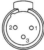
DMX - output XLR mounting-sockets (rear view):
