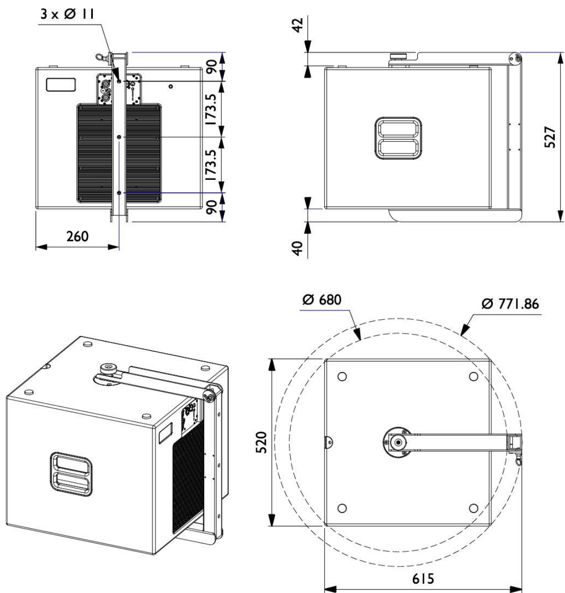
Figure 29: SB15P + ETR15P Line Drawing
