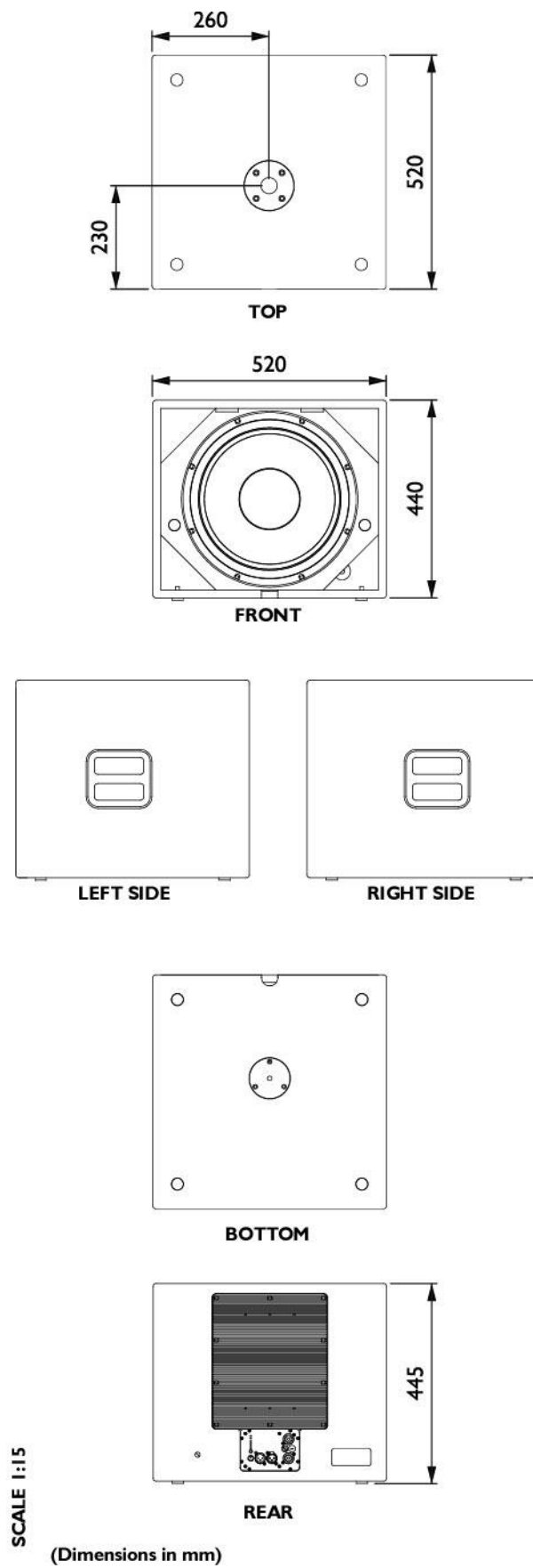
Figure 28: SB15P Line Drawing
